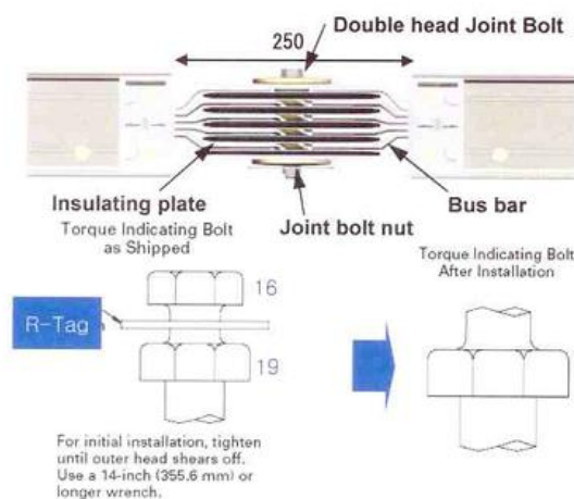
The side figure of bolt Fastening & Breaking
