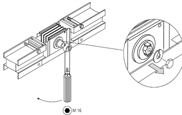
The side figure of bolt Fastening & Breaking
